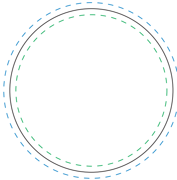
Circle 3.375" (3 3/8")
